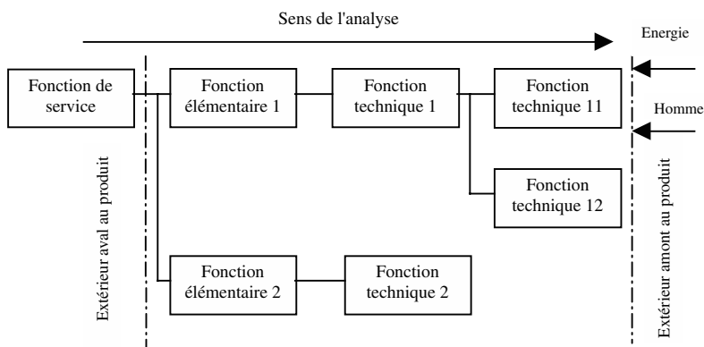
Figure 1.4 Diagramme FAST.
