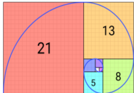
Fibonacci sequence. From wikipedia
