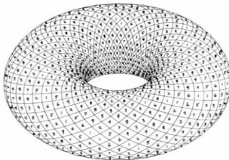
The Rodin Coil Vortex-Based Mathematics Toroid Surface Topology
